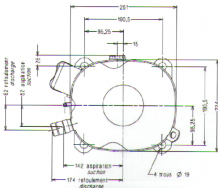
Detail suspension Echelle: 1/2 Scale: 1/2
