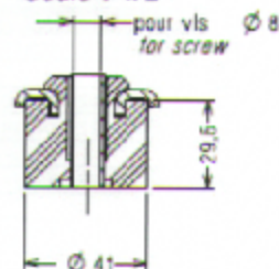
Detail suspension Echelle: 1/2 Scale: 1/2
